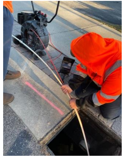
Crews Cleanout catch basin silt acks and camera stormwater pipes.
